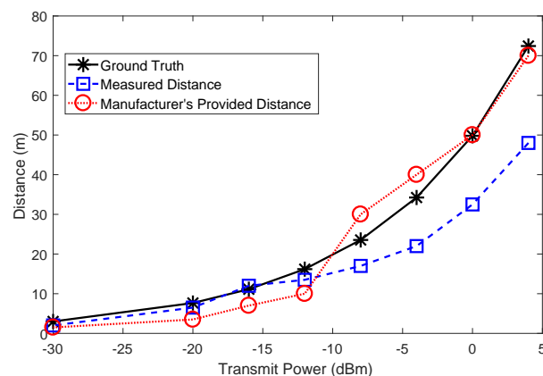
Fig. 3. Distance versus transmit power.
