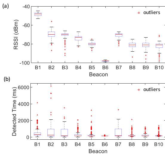
Fig. 4. Variation in BLE beacon signal characteristics in a dense environment: (a) the RSS; (b) the time interval to detect a beacon signal.
